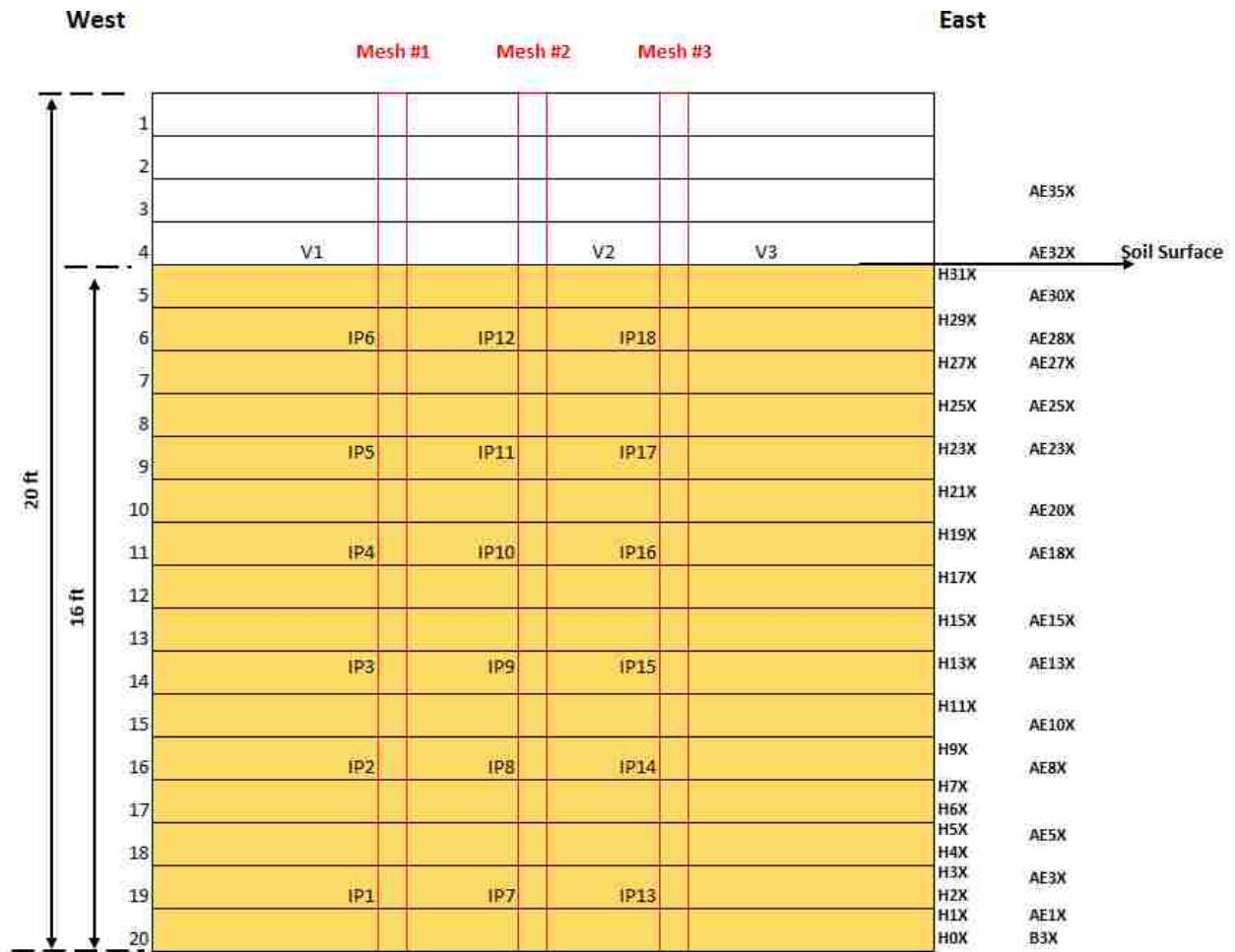
Figure 74 Profile View of Sensors Installed for PVD-2
