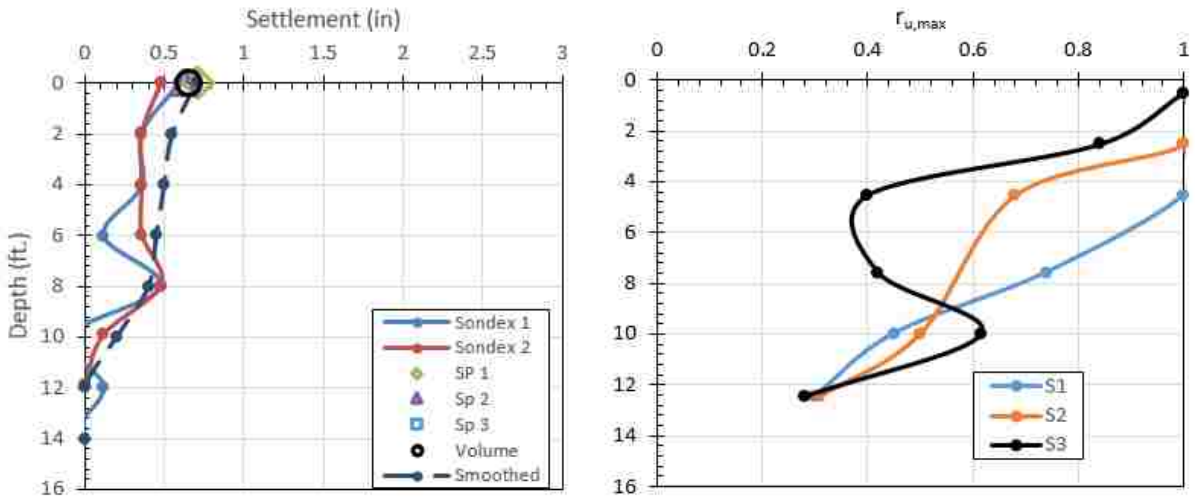
Figure 57 Profiles of Liquefaction Induced Settlement and Maximum Excess Pore Pressure Ratio ( r_{u,max} ) for Round 3 Test with a_{max}=0.10 g.
